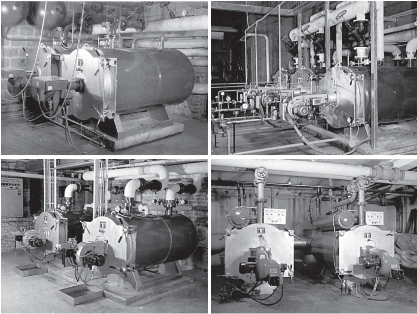
Enkele ketelinstallaties.
